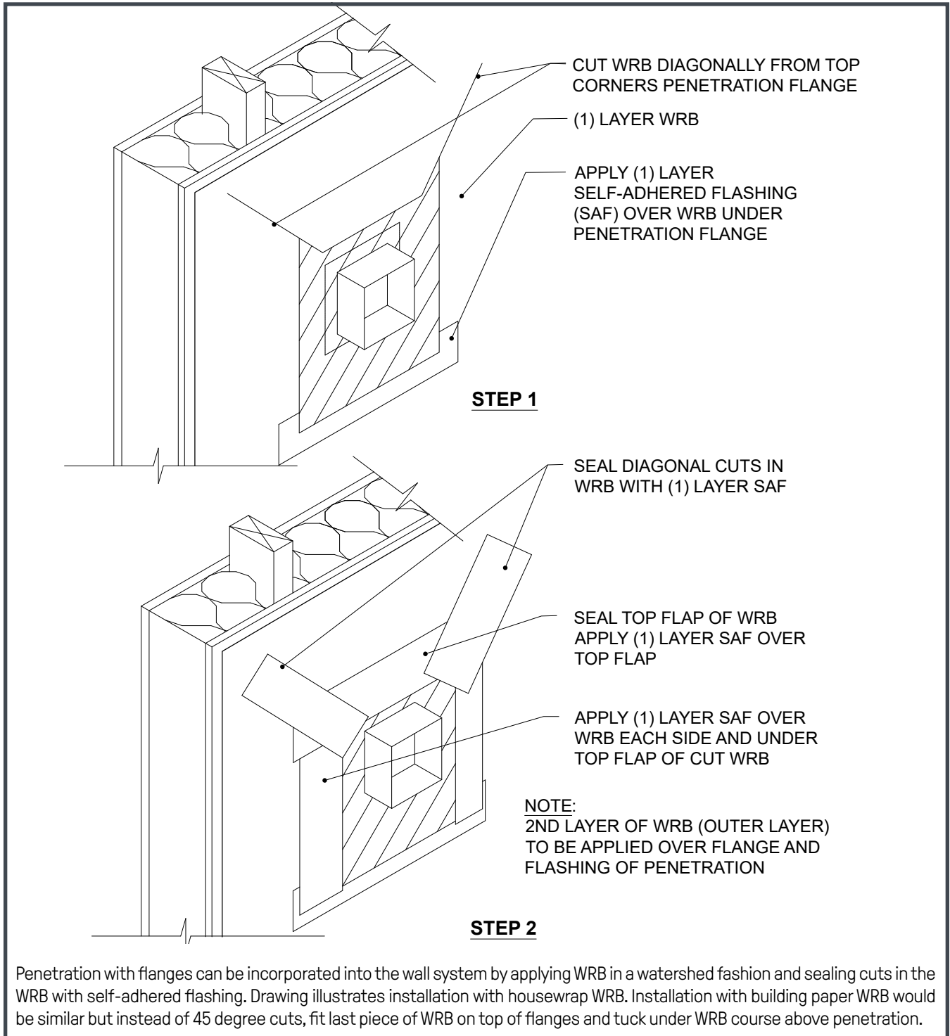
Figure 28. Penetration, Flanged
