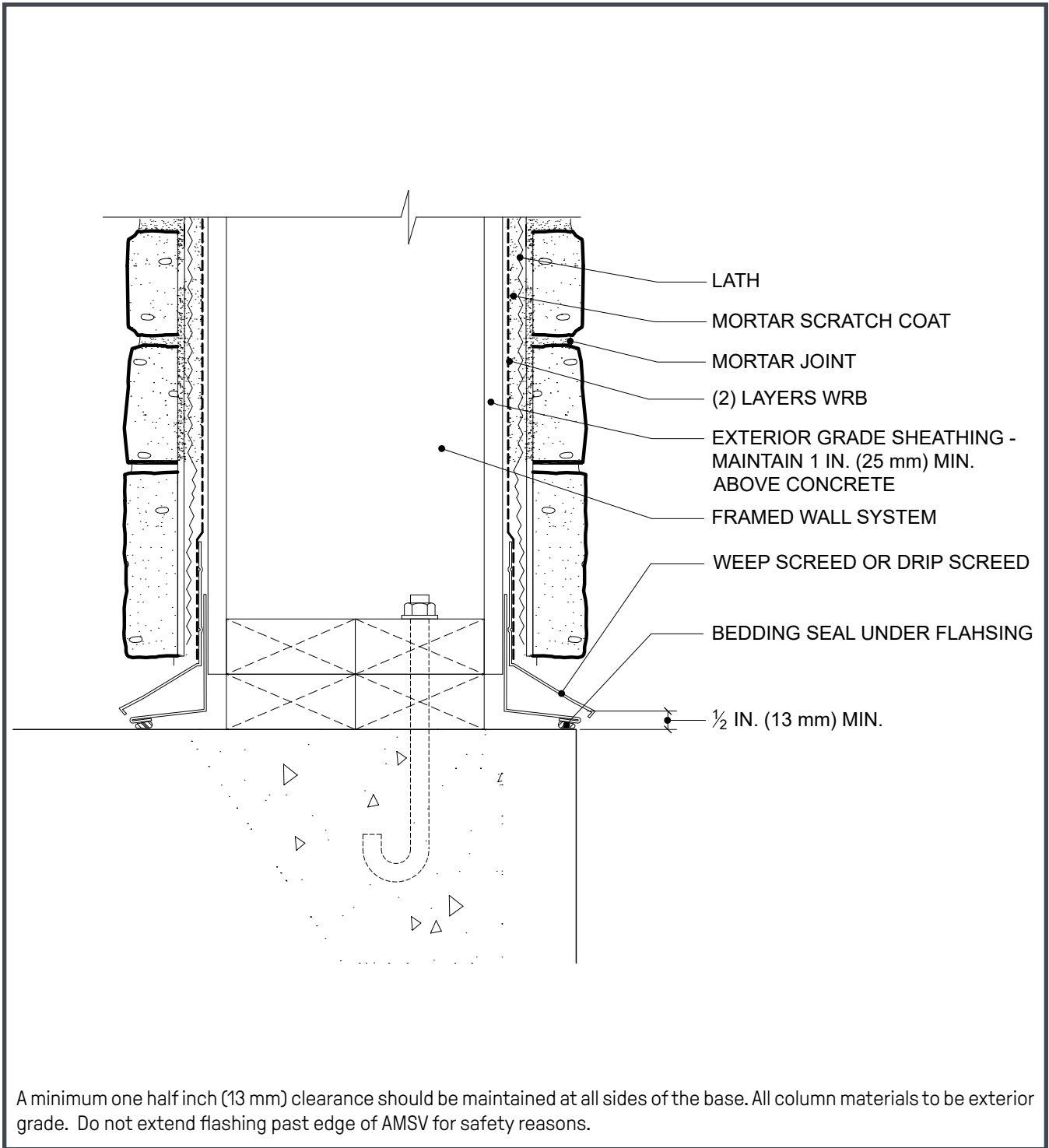
Figure 27. Column Base
